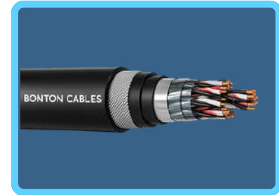
Control & Instrumentation Cables
